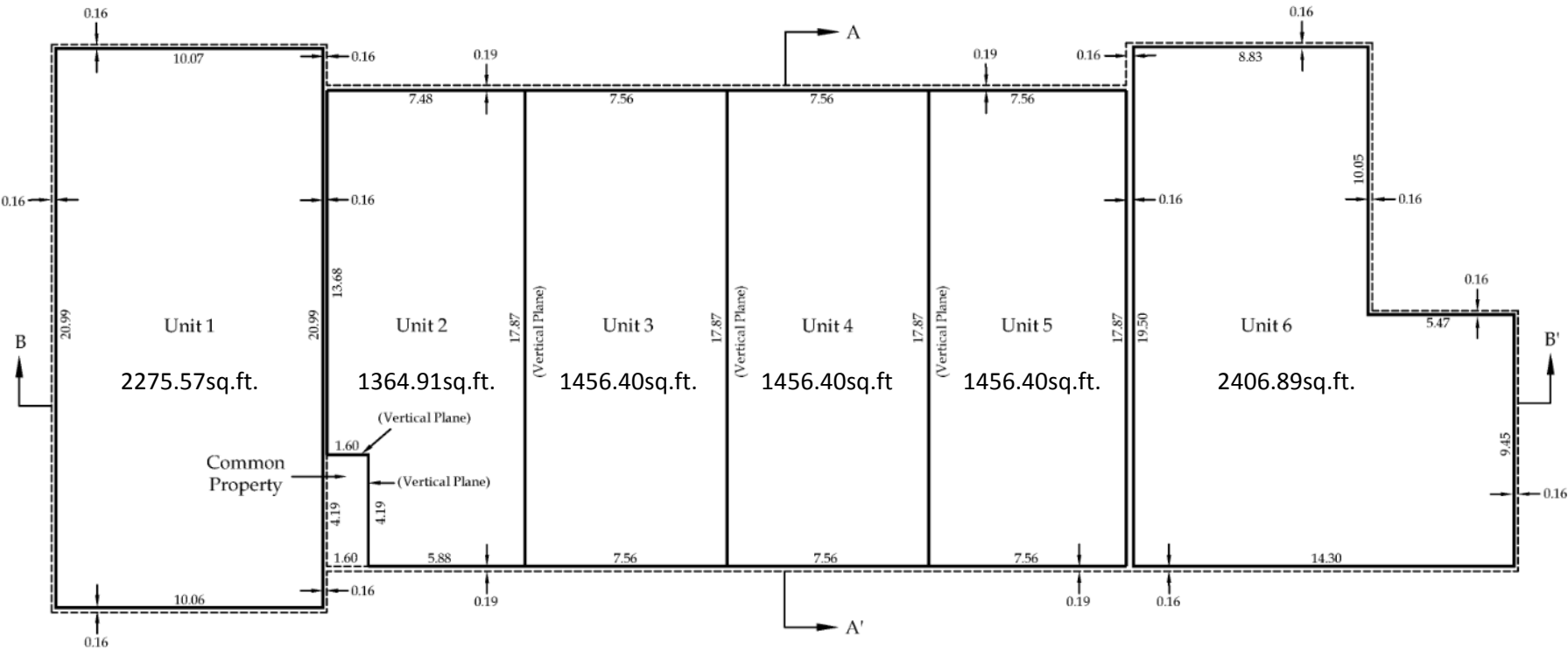
Main Floor Detail 0 2 4 8 12 metres Scale 1:200
